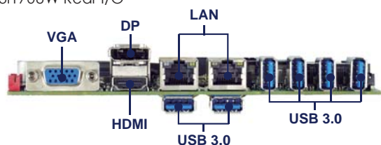
3I170UW Rear I/O
